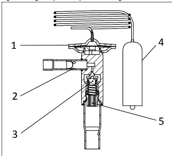
Figure 1: Angle way fixed superheat setting
